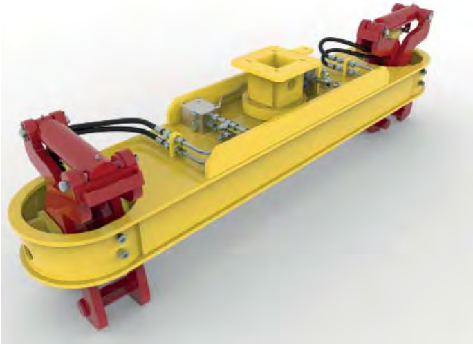
Example: UB02-01-05-01 Universal Lifting Beam, standard gauge, with Archimedes square drive head and no stillage
