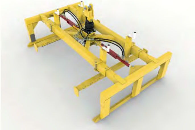
Example: CSH09-06-06 Six-Sleeper Handler with rotator and truck mounted crane adapter.
